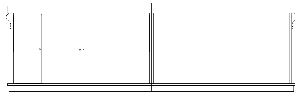
Front bar - rear
