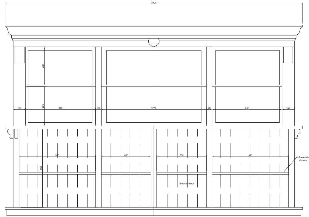
Back bar - front
