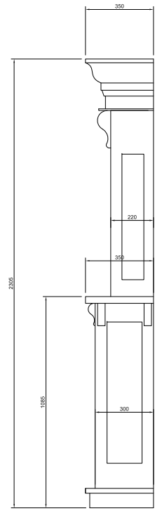
Back bar - side
