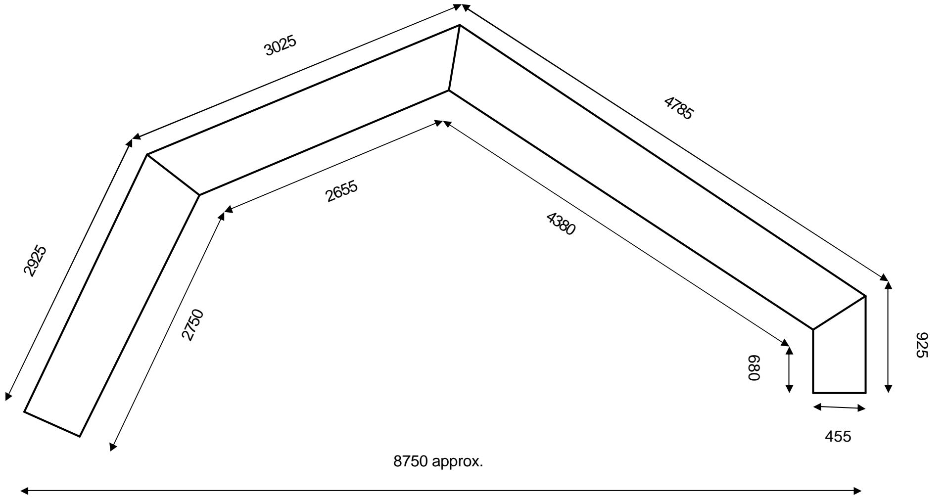
ATVM BAB 0123 Mahogany corner bar counter Plan not to scale. All dimension are in mm
