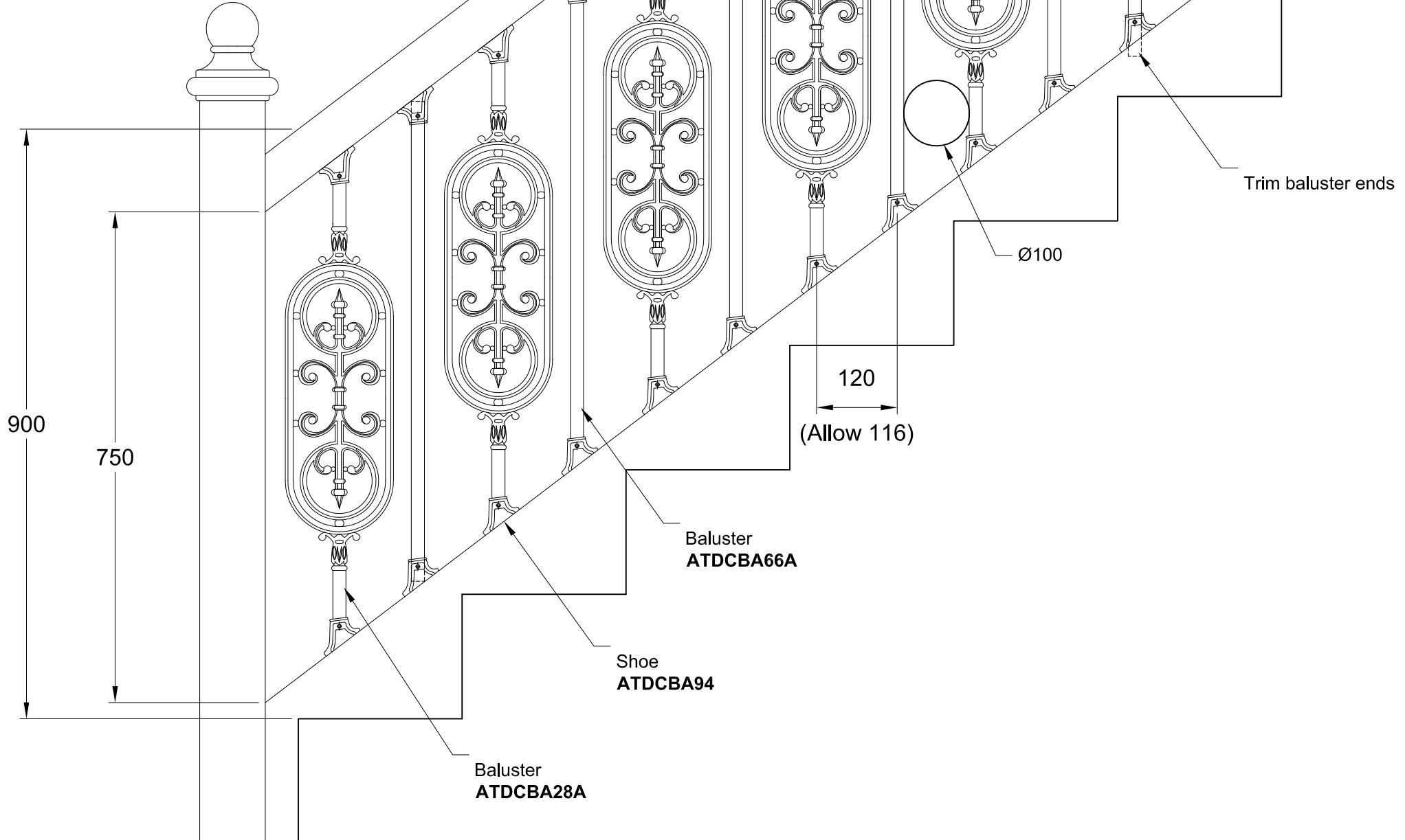
BALUSTER ATDCBA28 (ON TYPICAL STAIR) REGULATION CLEARANCE
