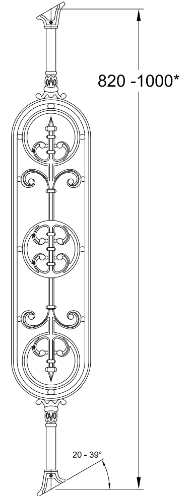
WITH ANGLED BALUSTER SHOES ATDCBA94
