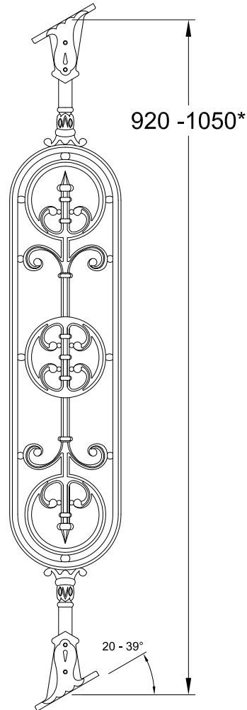
WITH ANGLED BALUSTER BRACKETS ATDCBA34
