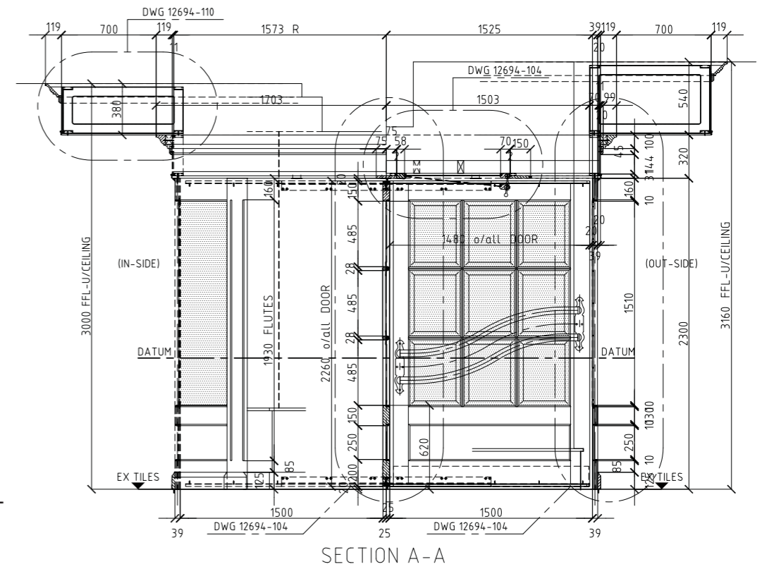
Elevation detail, KEMPINSKI HOTEL GRAND ARENA
